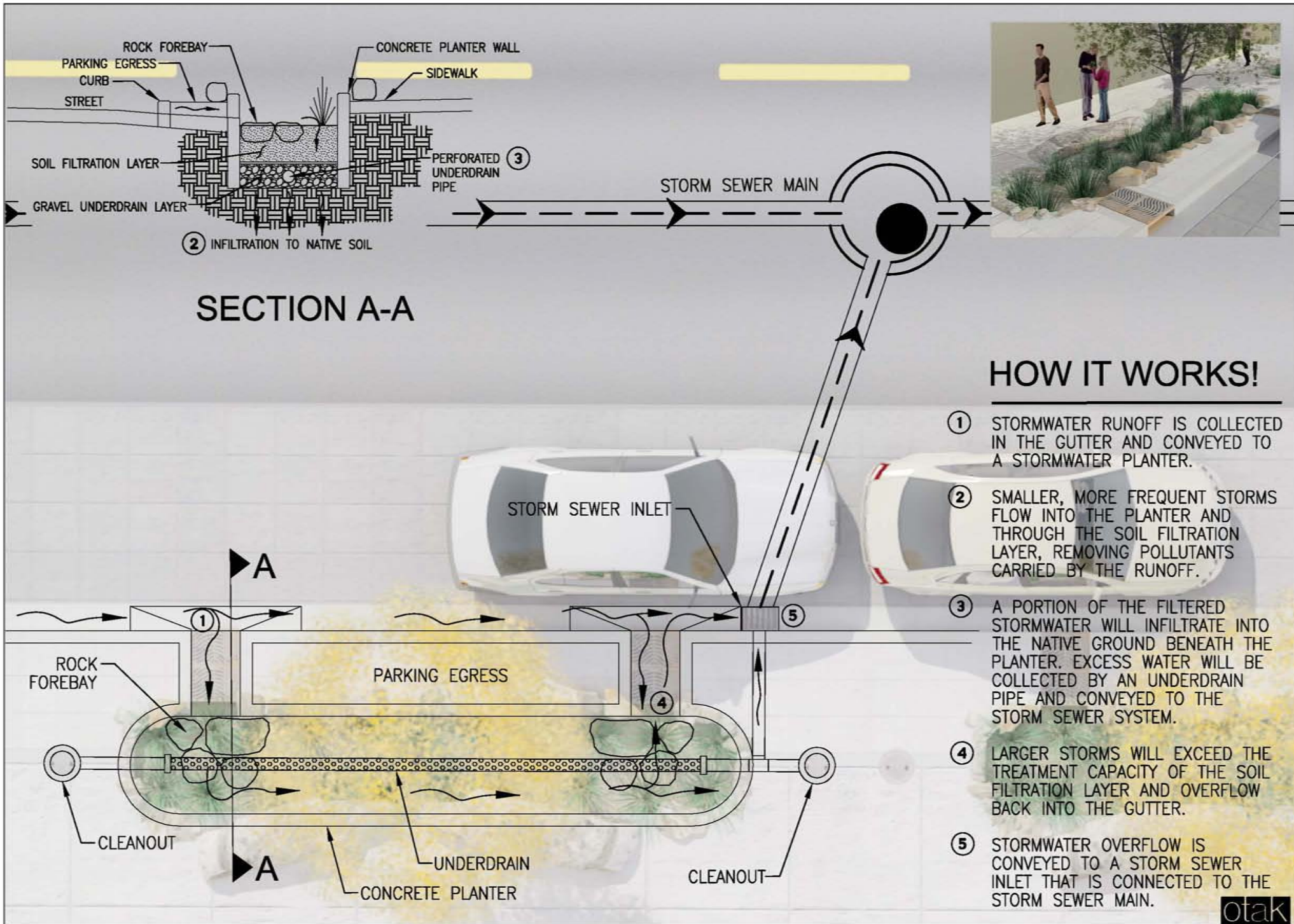
FLOW THROUGH SIDEWALK PLANTER
