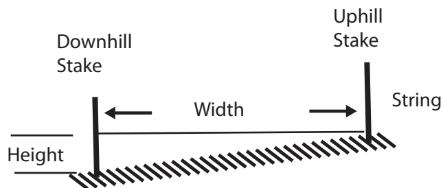
Figure 2: Calculating Slope
