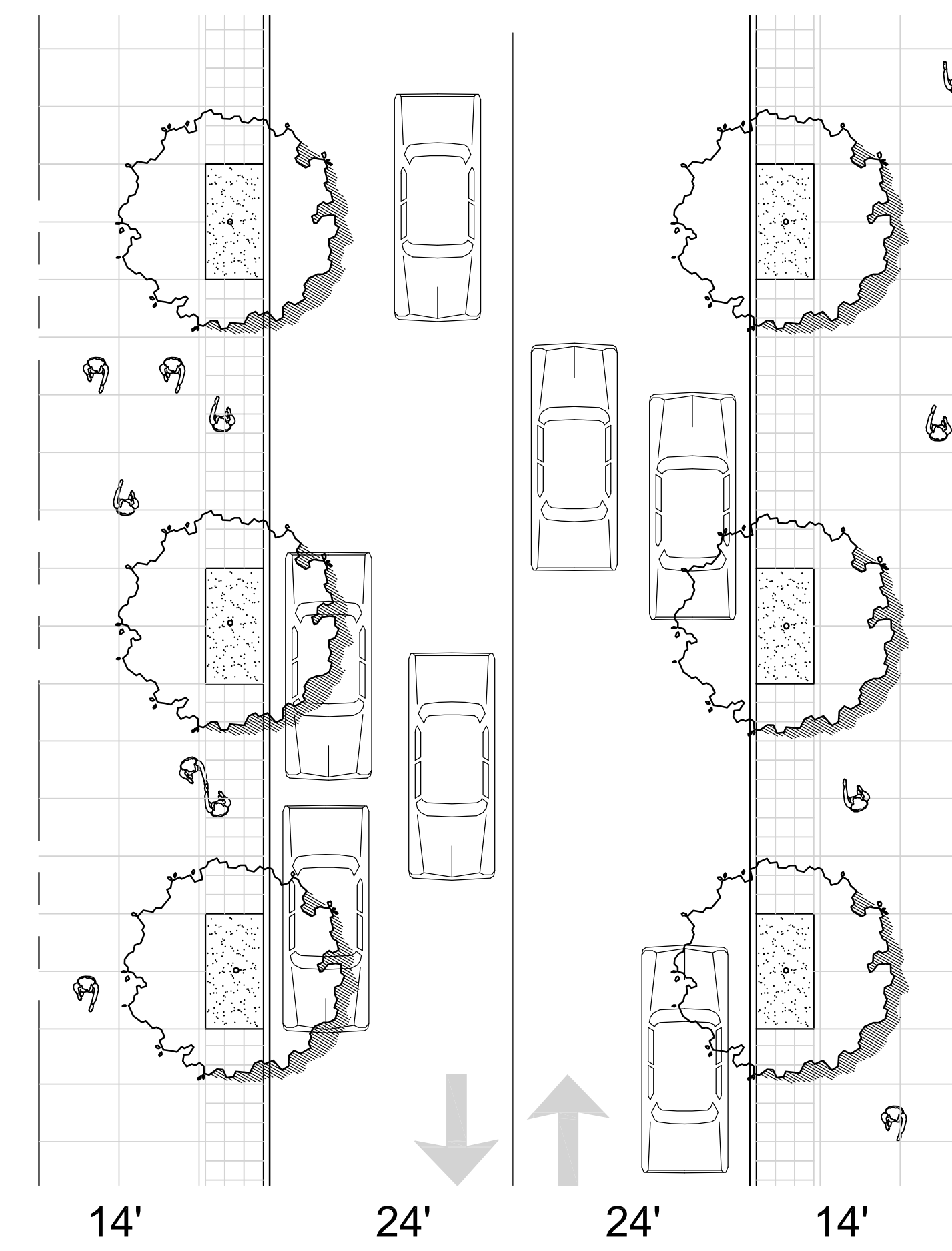
ASH STREET South Section
