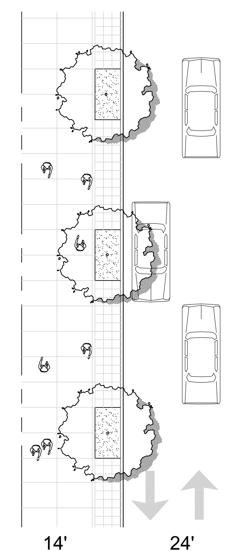
ASH STREET North Section
