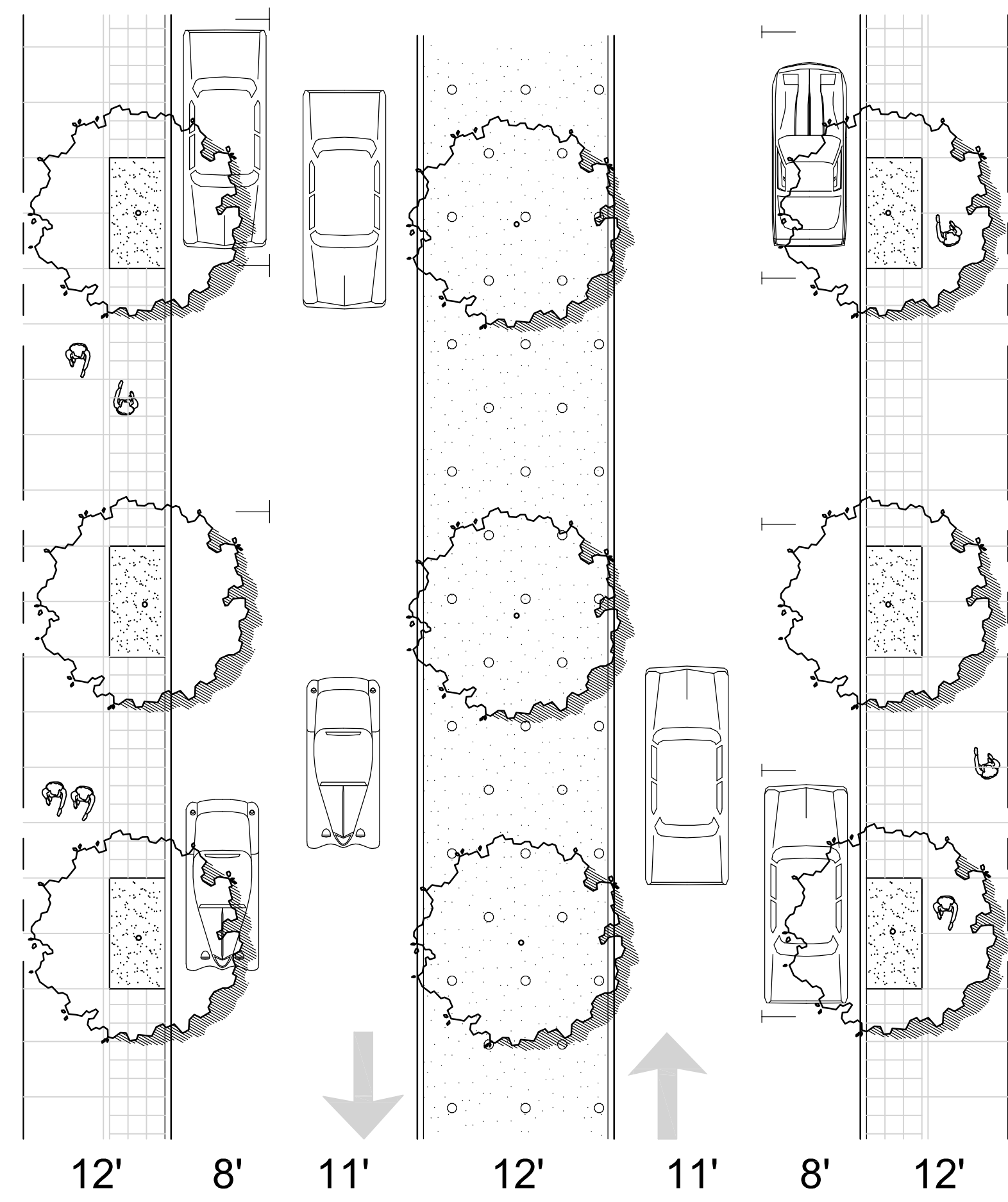
BURNHAM STREET Ash to Hall Section
