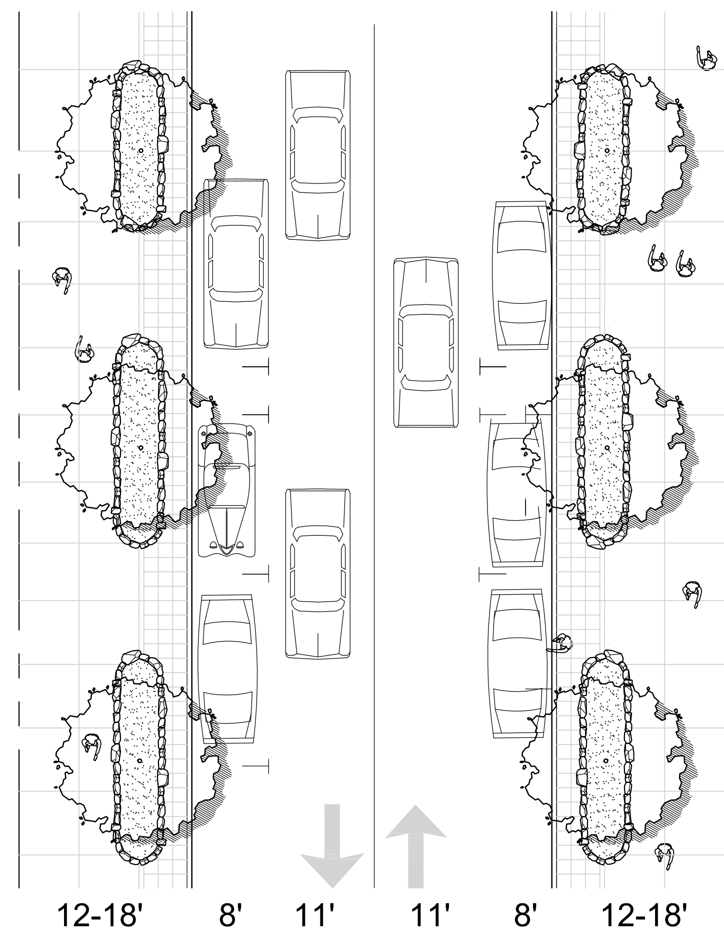
BURNHAM STREET Main to Ash Section
